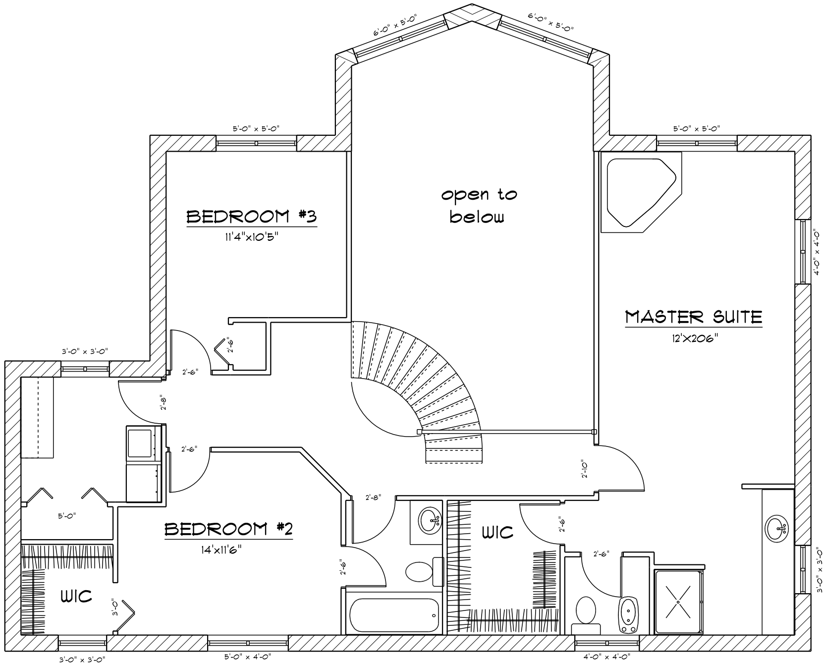
TOP FLOOR LAYOUT 1158 SQ. FT.
