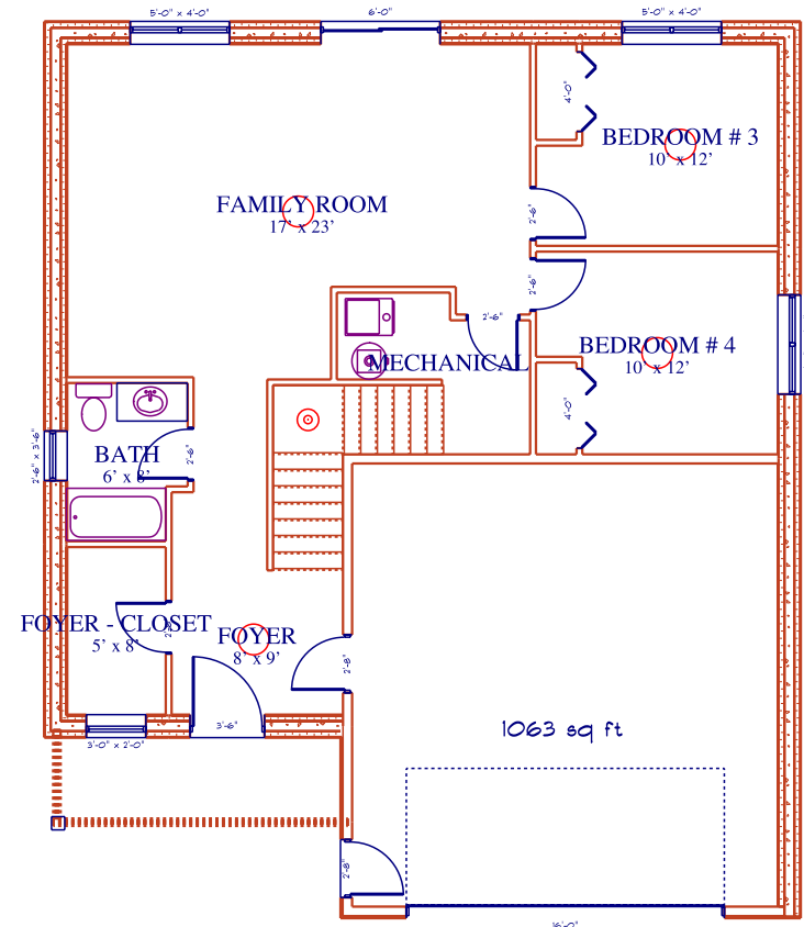
Basement
