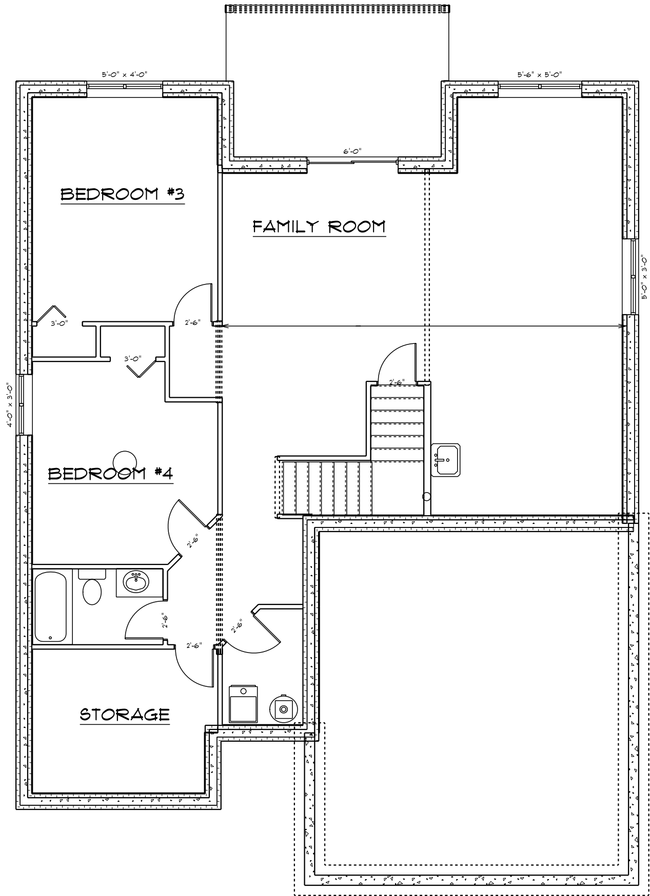
BASEMENT PLAN 1472 sq ft
