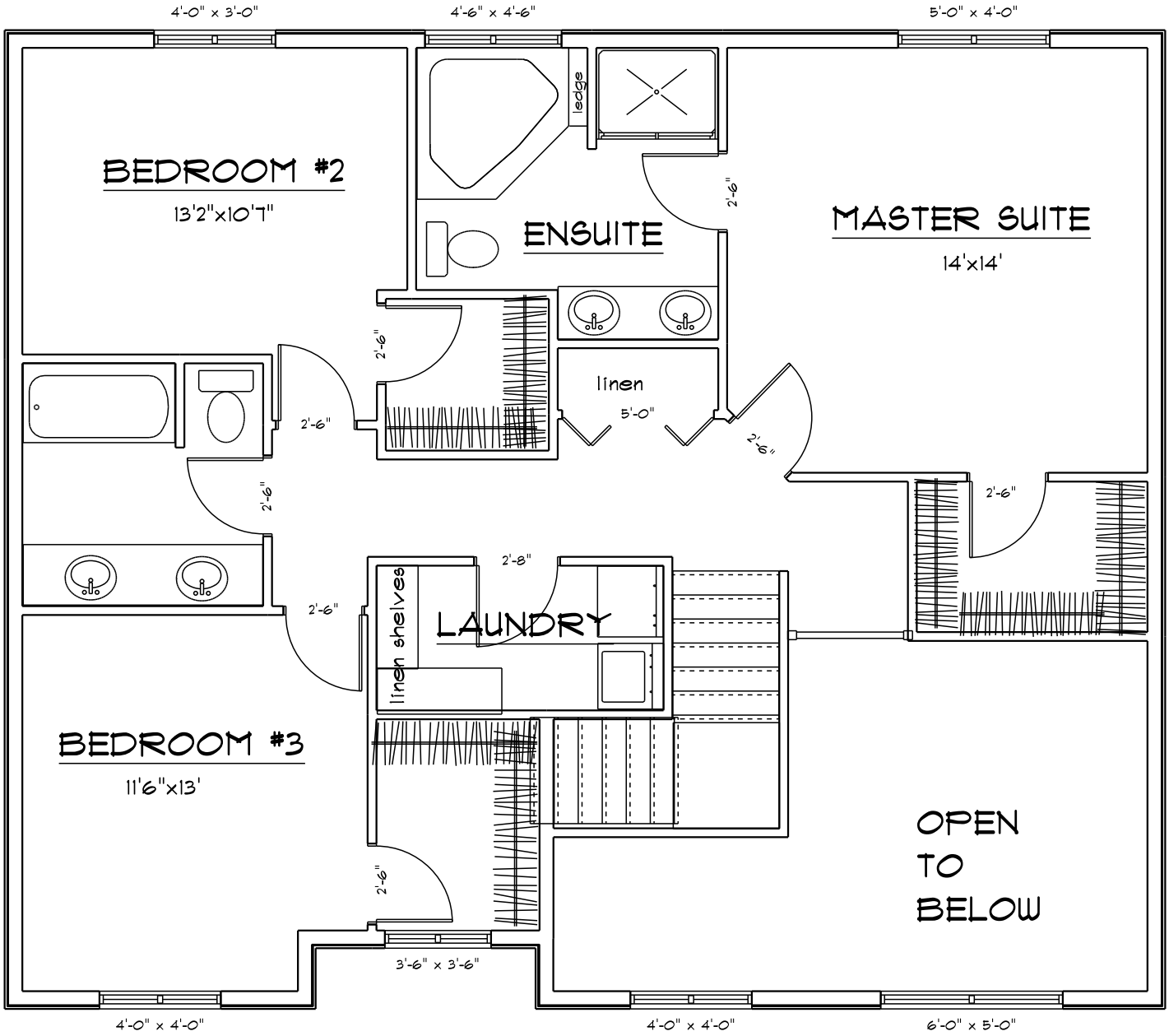
TOP FLOOR PLAN 890 sq. ft.
