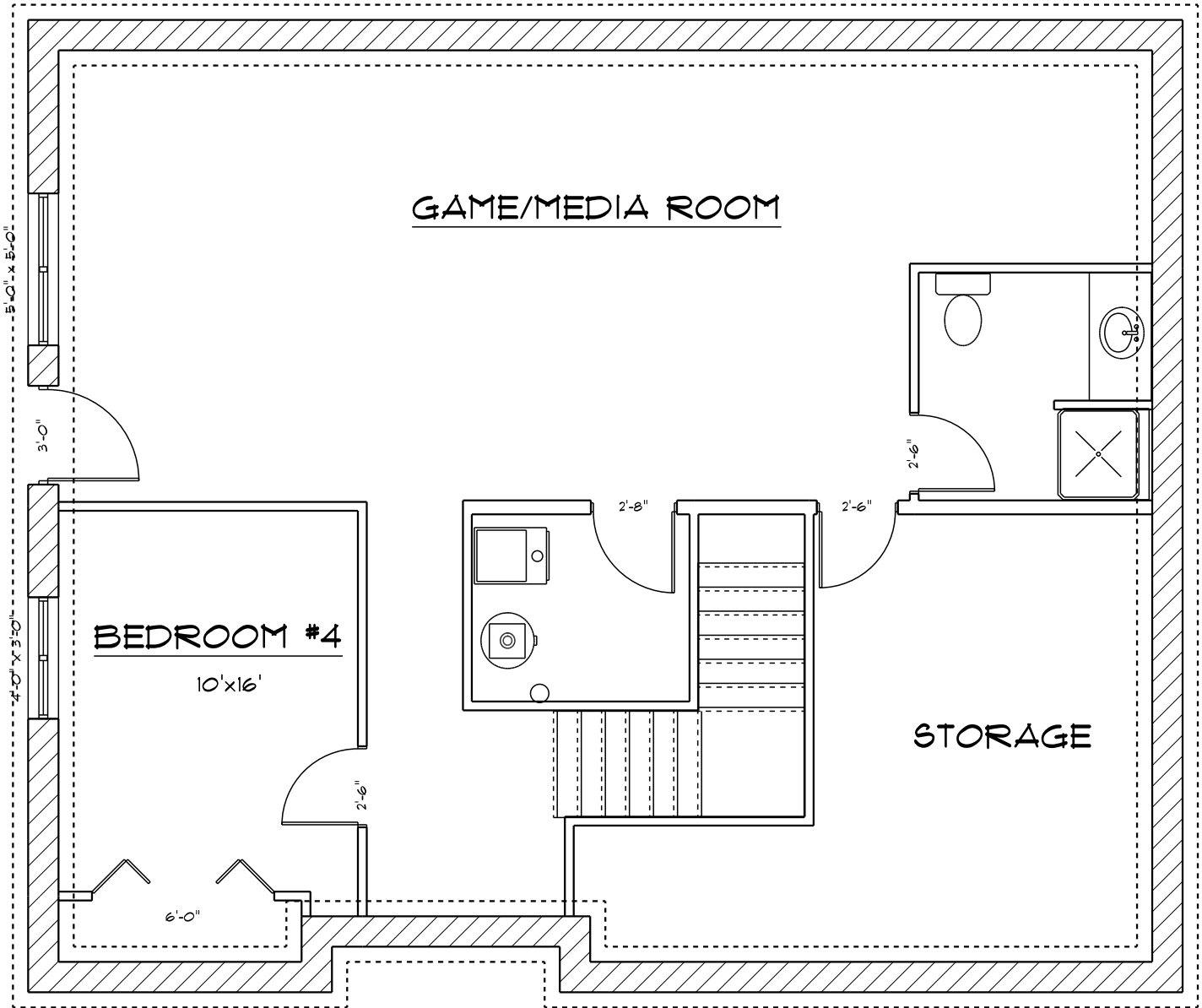
FUTURE BASEMENT LAYOUT
